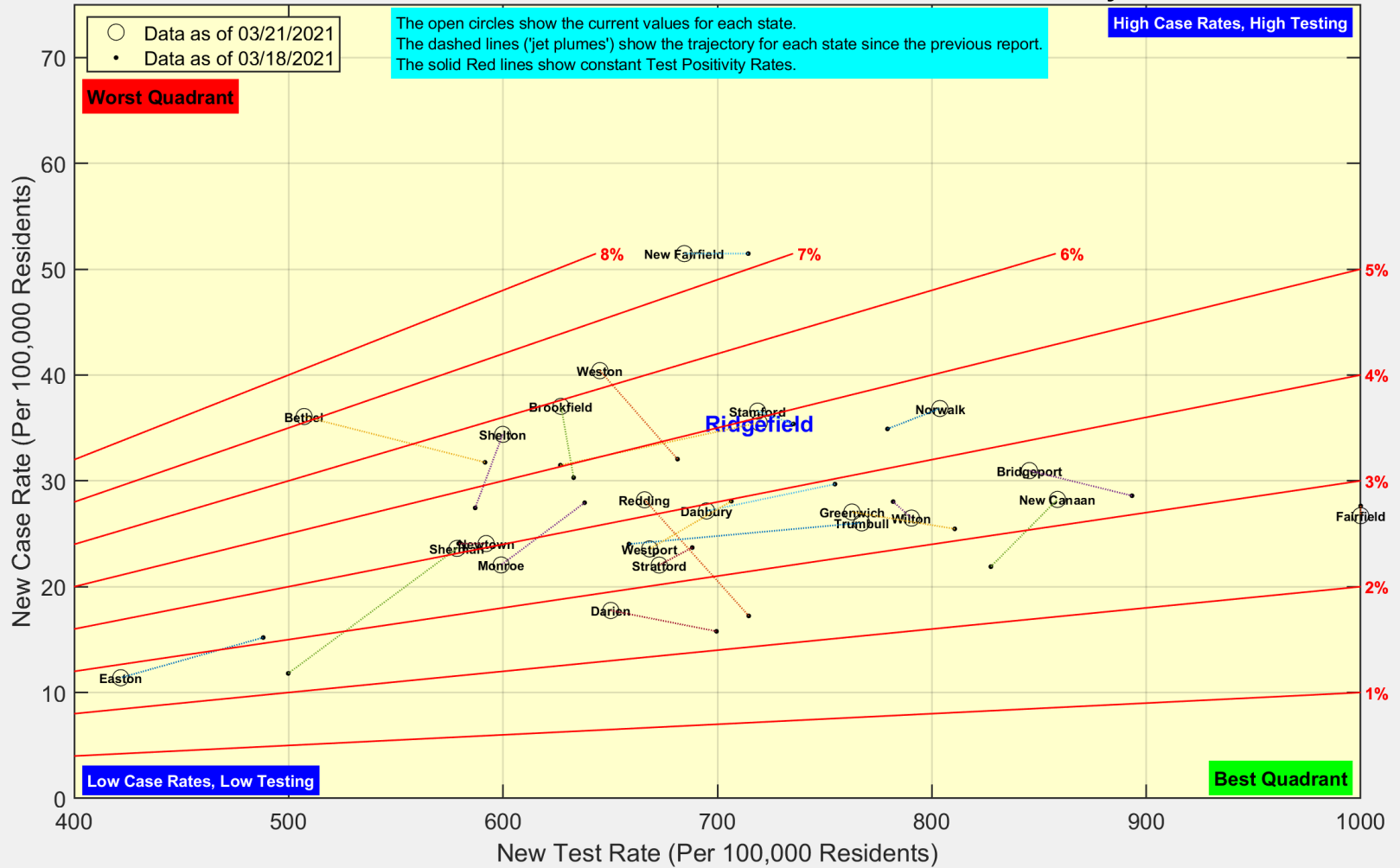
New Case Rate vs New Test Rate for all Towns in Fairfield County
